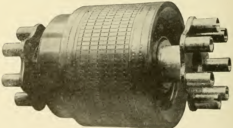
Fig. 258. View of Hollow Armature Shaft and Pin Plate
